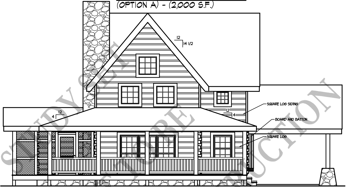
FRONT ELEVATION
