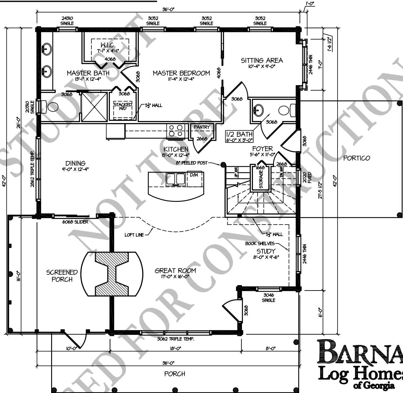
1st FLOOR PLAN (OPTION A) - (1,311 S.F.)
