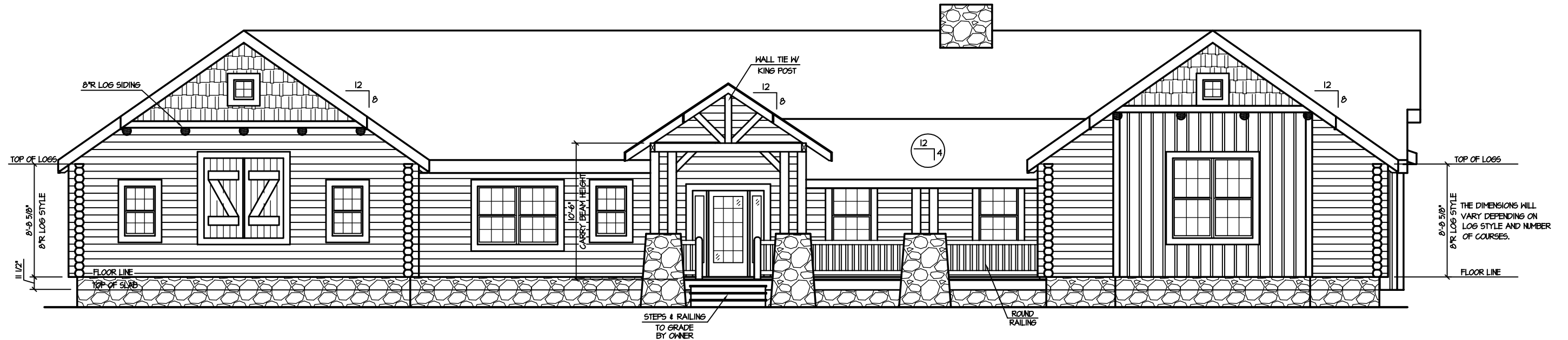
FRONT ELEVATION
