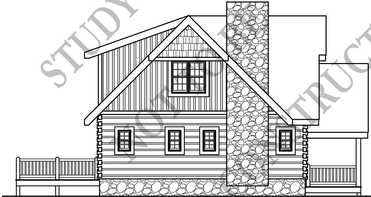
LEFT ELEVATION
