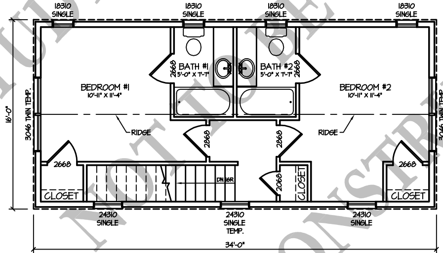
2nd FLOOR PLAN (544 S.F.)
