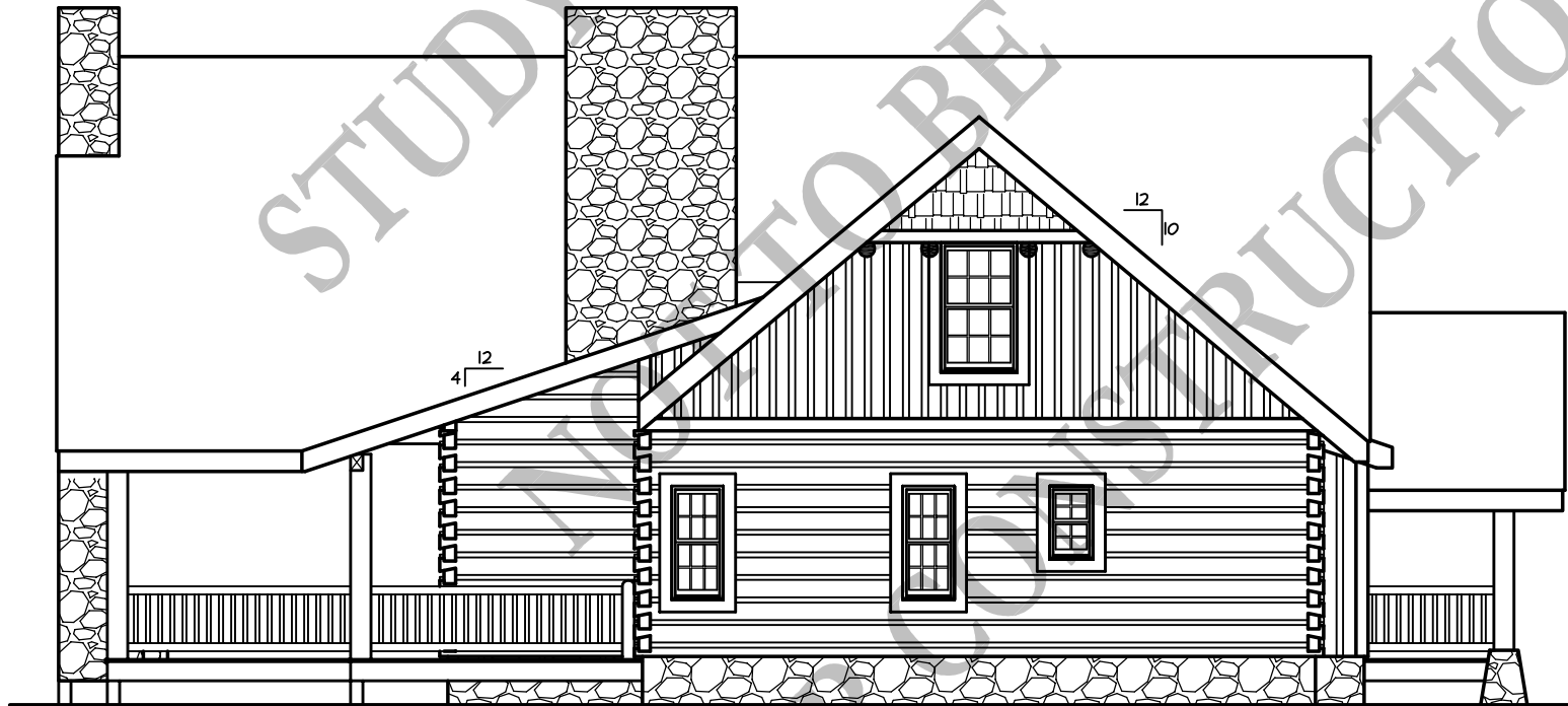
LEFT ELEVATION
