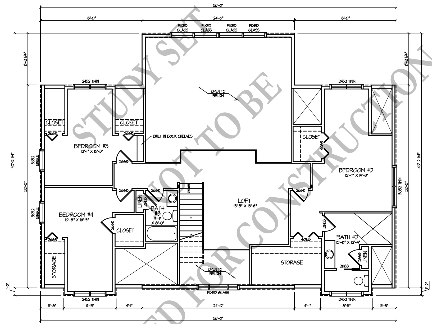
2nd FLOOR PLAN (1,196 S.F.) 1/8" = 1'-0"
