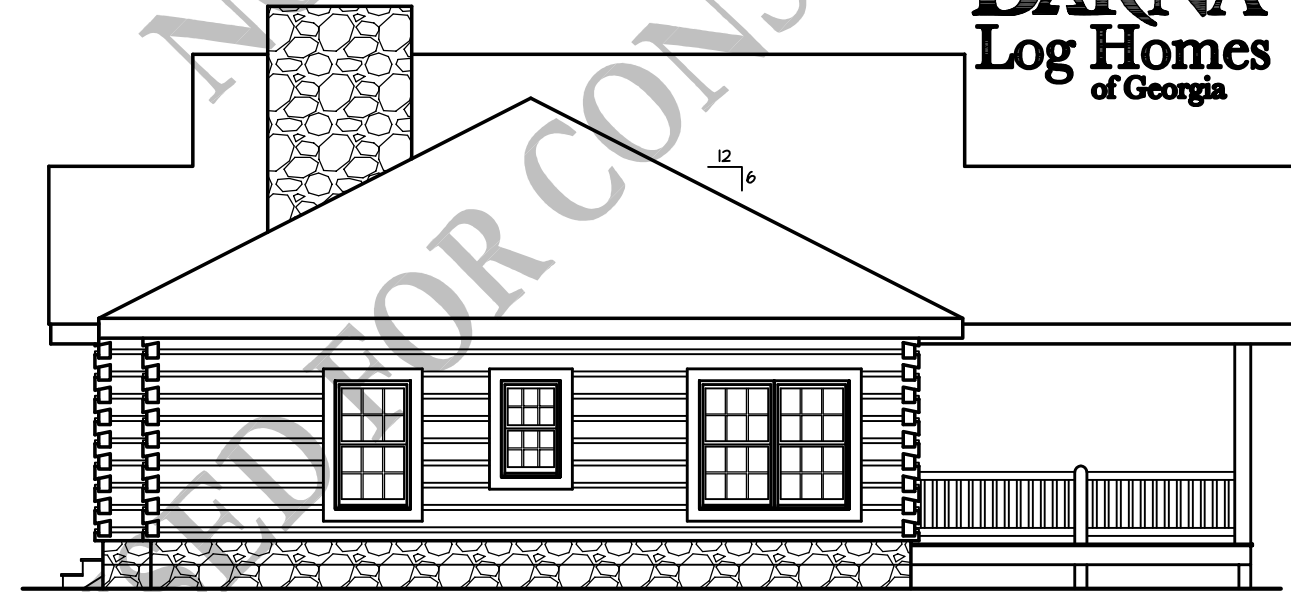
RIGHT ELEVATION 1/8" = 1'-0"
