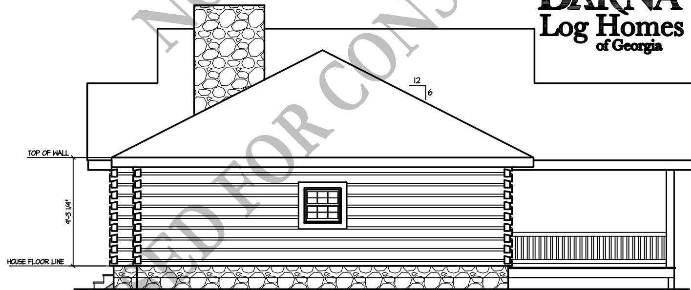
RIGHT ELEVATION 1/8" = 1'-0"
