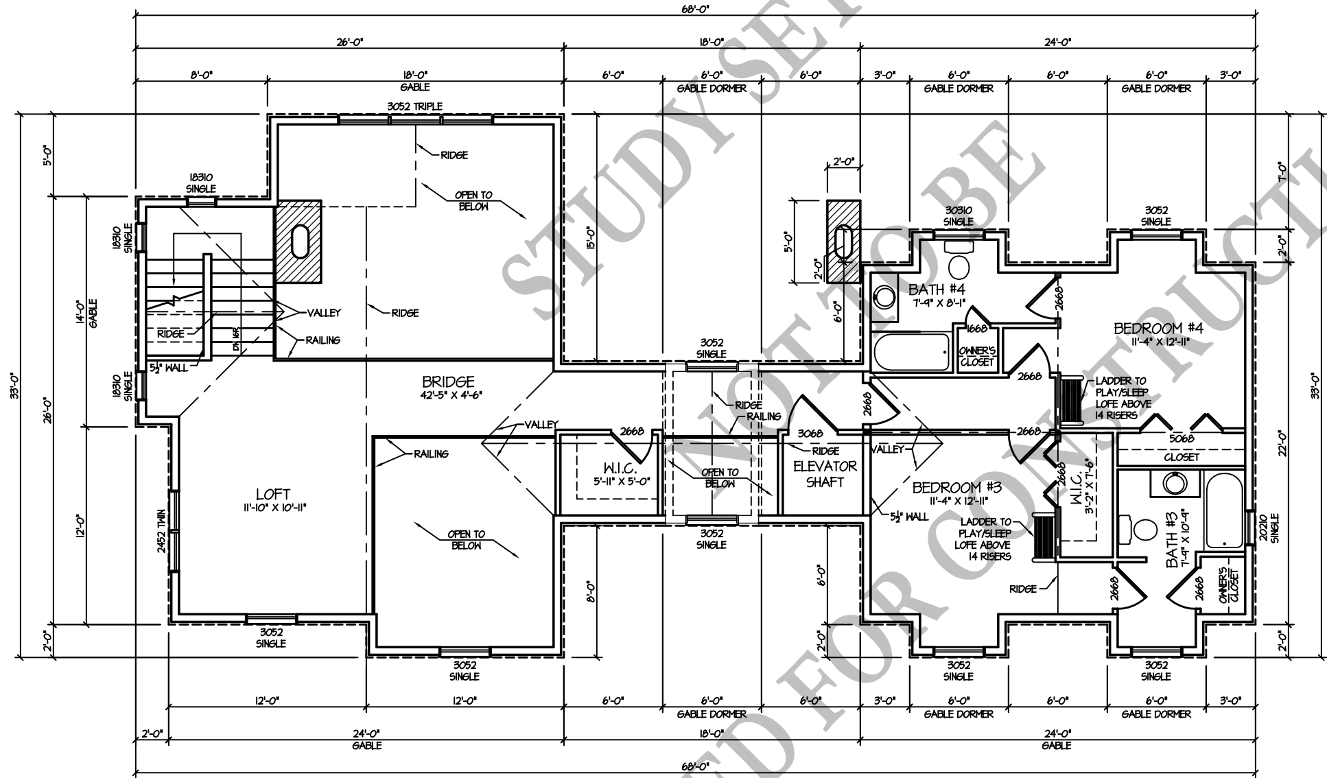
2nd FLOOR PLAN (938 S.F.)
