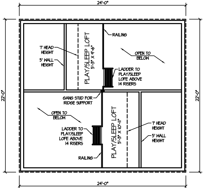
PLAY LOFT DETAIL (125 S.F.)
