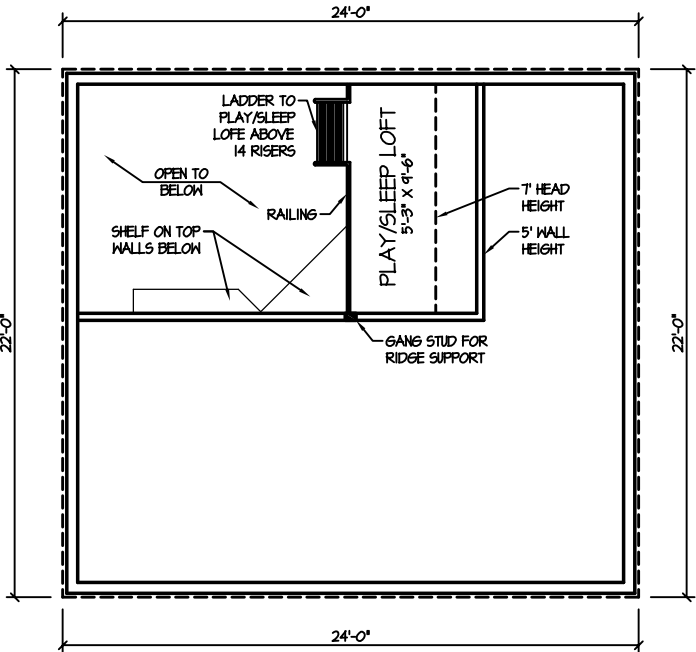
PLAY LOFT DETAIL (54 S.F.)
