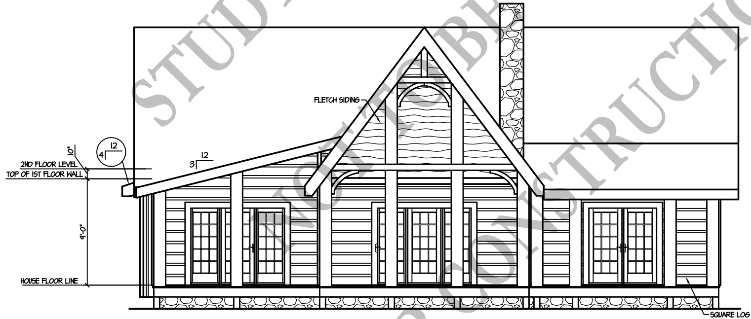
REAR ELEVATION
