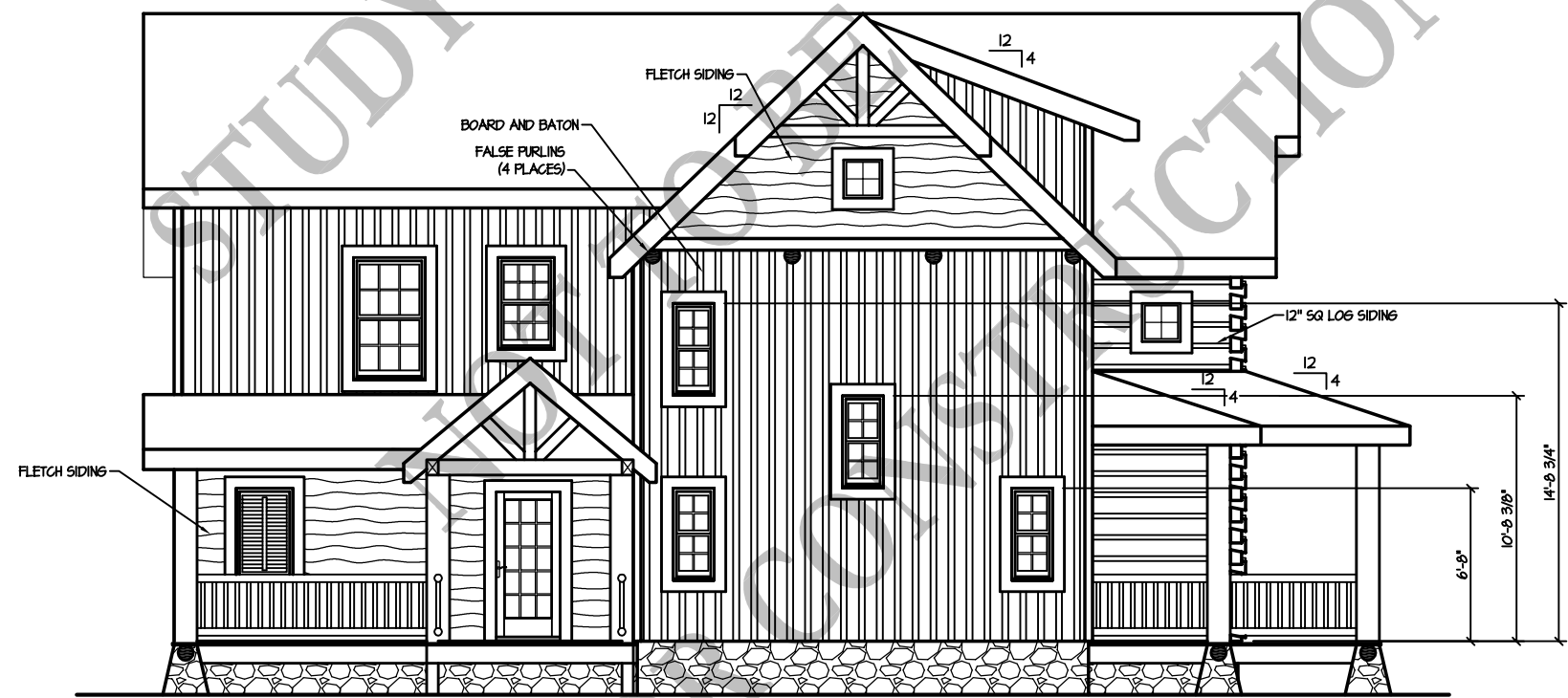
LEFT ELEVATION
