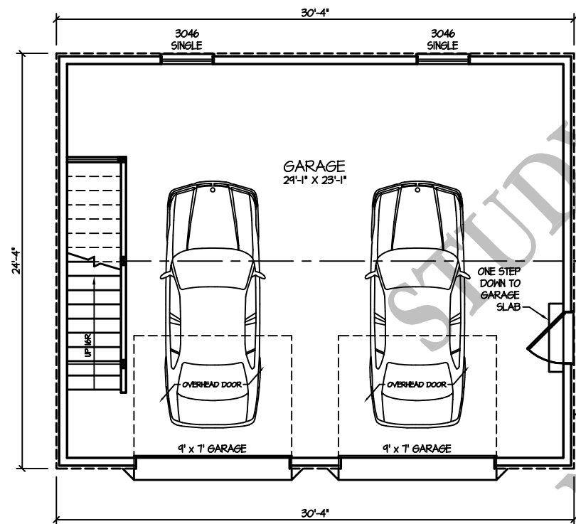
1st FLOOR PLAN (GARAGE)
