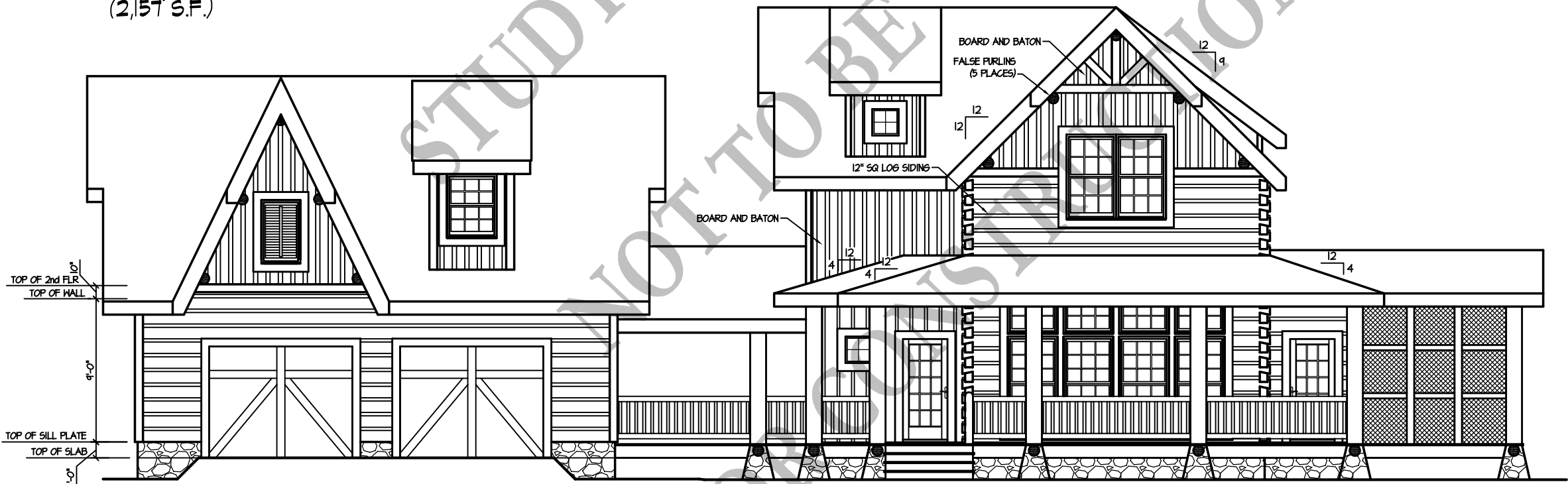
FRONT ELEVATION
