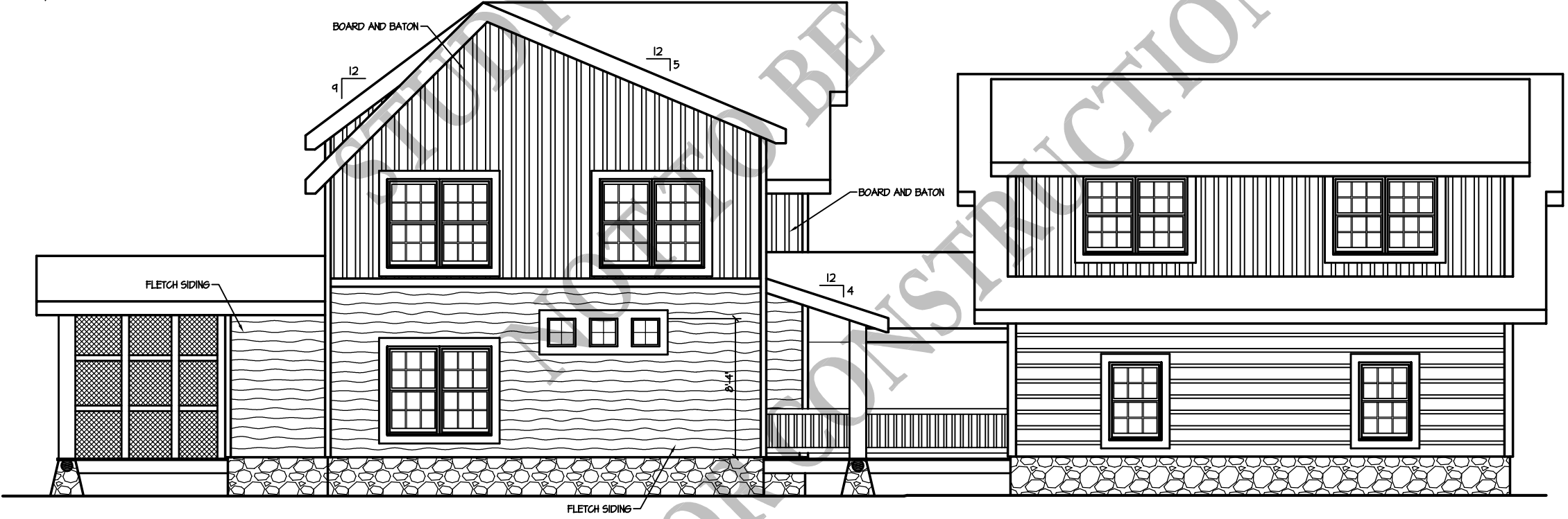
REAR ELEVATION
