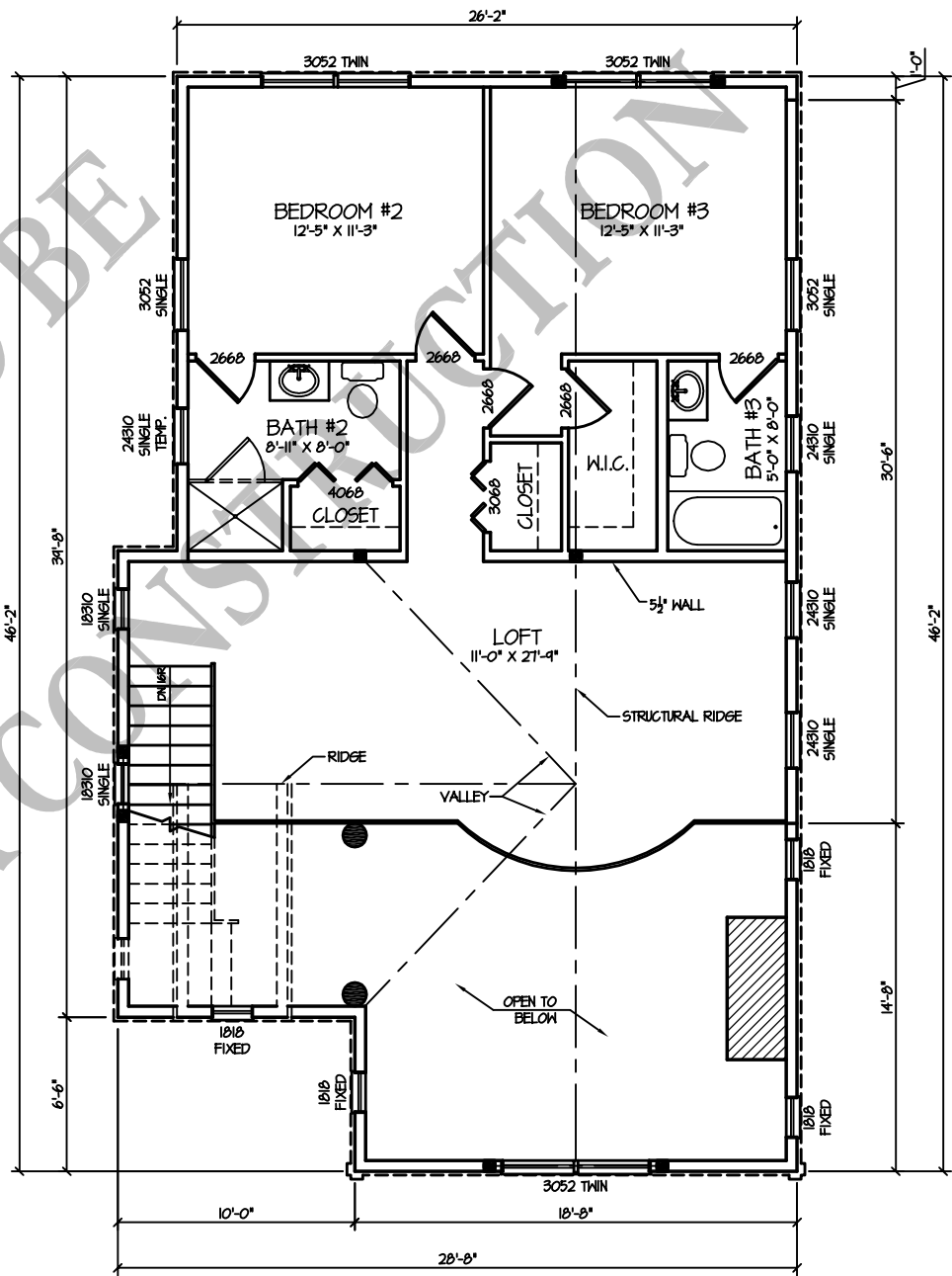
2nd FLOOR PLAN (867 S.F.)
