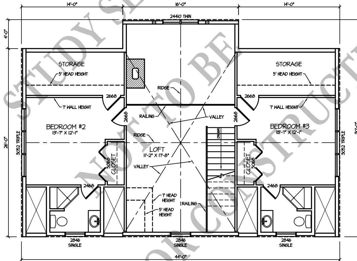
2nd FLOOR PLAN (744 S.F.)
