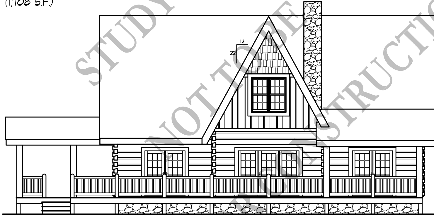
REAR ELEVATION
