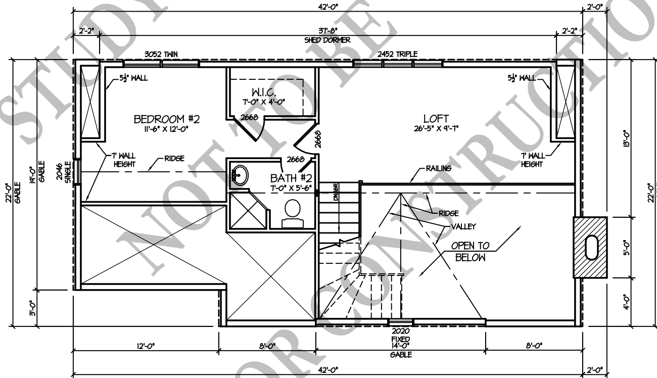
2nd FLOOR PLAN (463 S.F.)
