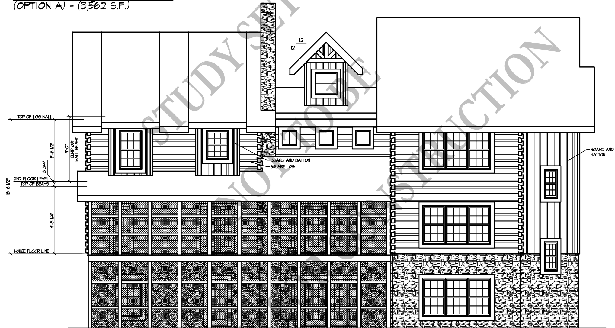
REAR ELEVATION OPTION A
