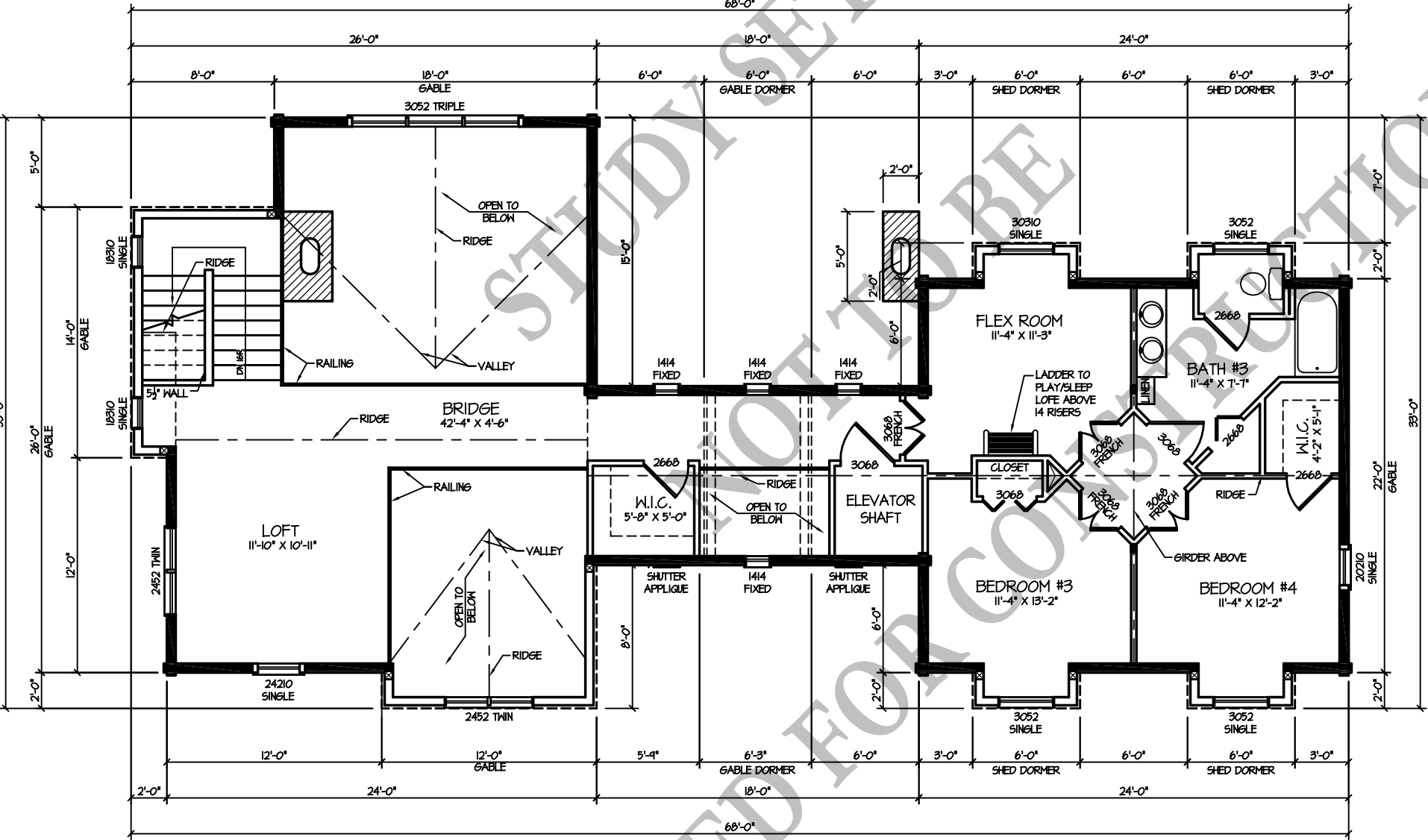
2nd FLOOR PLAN (987 S.F.) 1/8" = 1'-0"
