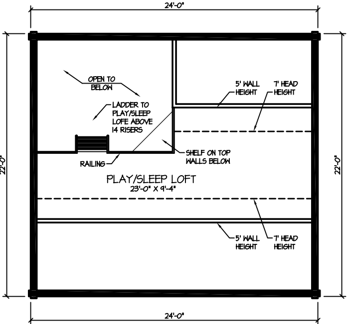
PLAY LOFT DETAIL OPTION B - (191 S.F.) 1/8" = 1'-0"
