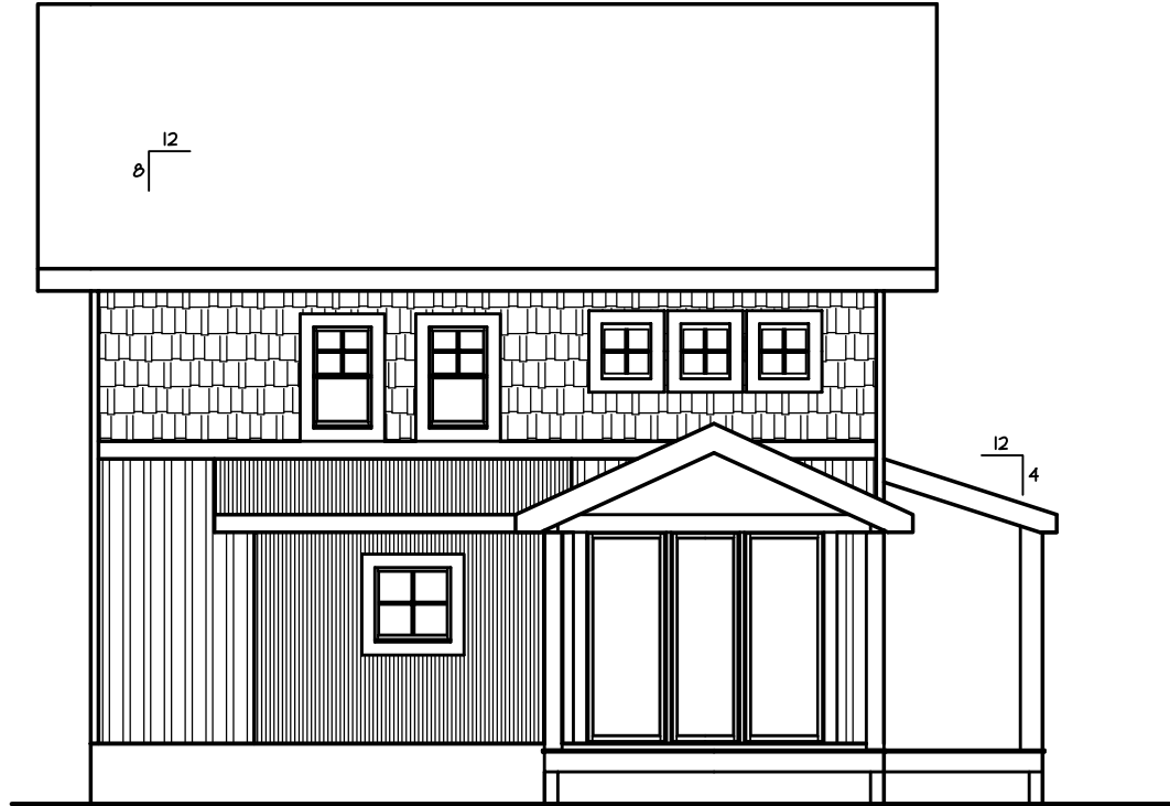
LEFT ELEVATION
