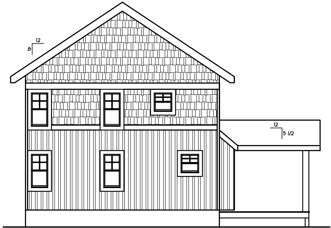
REAR ELEVATION
