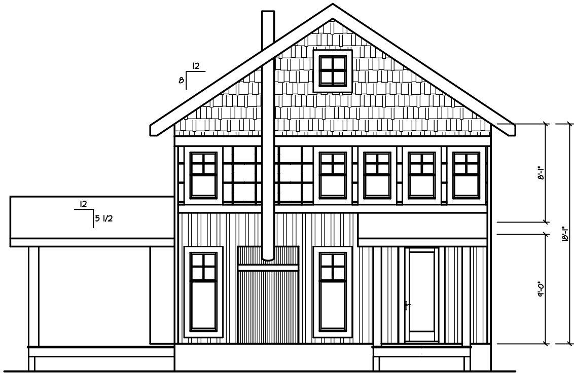
FRONT ELEVATION
