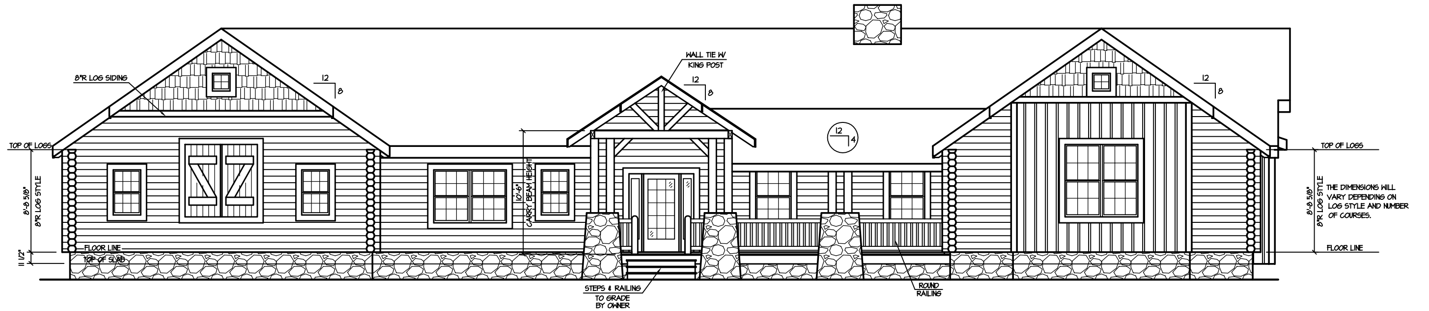
FRONT ELEVATION 1/8" = 1'-0"
