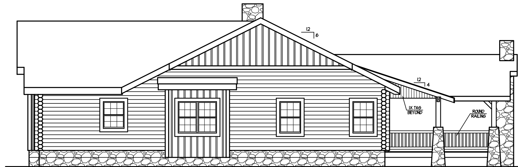
RIGHT ELEVATION 1/8" = 1'-0"
