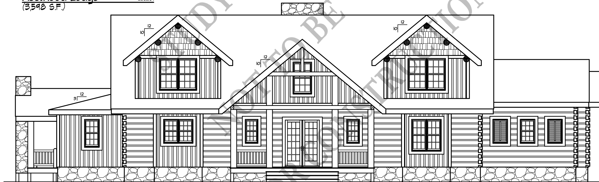
FRONT ELEVATION 1/8" = 1'-0"
