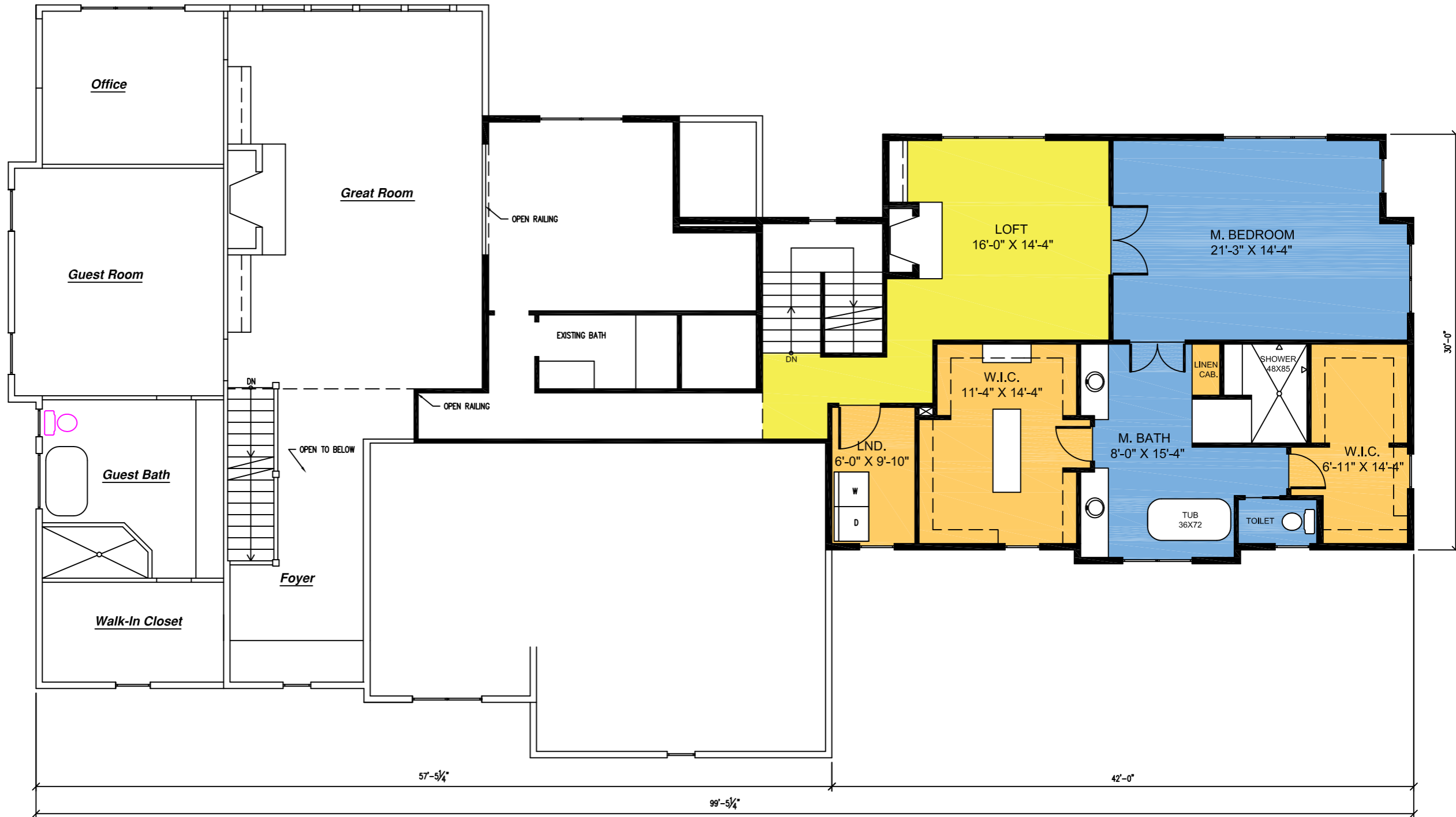
Loft Floor Plan
