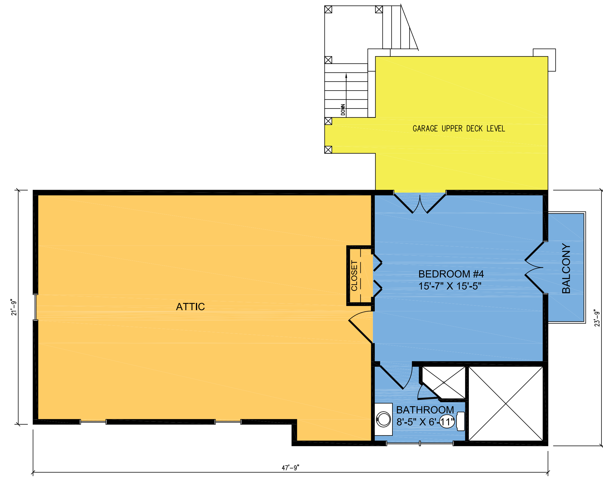
2nd FLOOR PLAN 1/4" = 1'-0"
