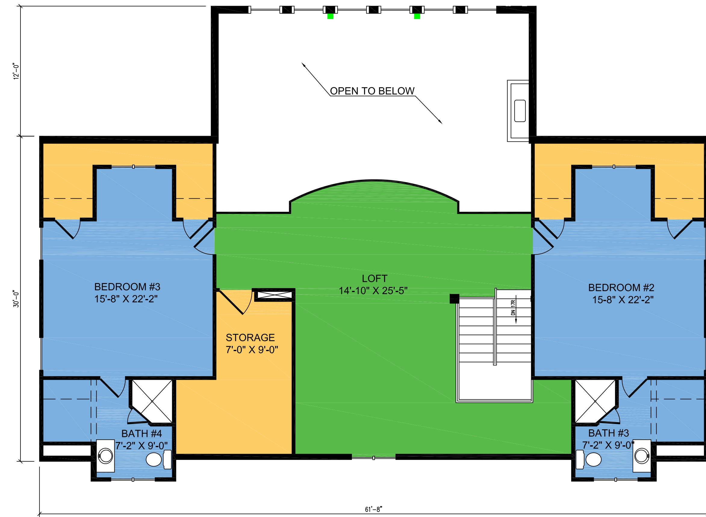
2nd FLOOR PLAN 1/4" = 1'-0"
