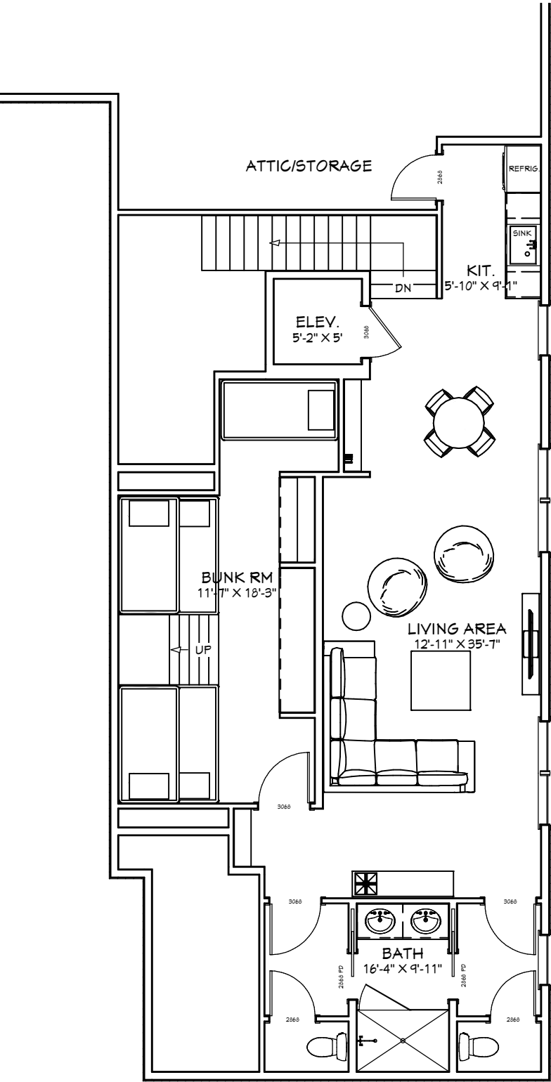
Garage Apt. Plan Scale: 1/8" = 1'-0"
